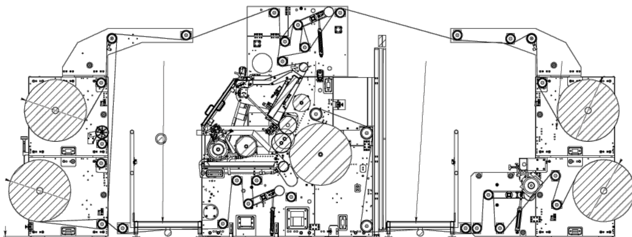
Multi-unwinder
